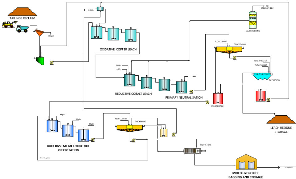
Figure 2: Kipushi Process Flowsheet
